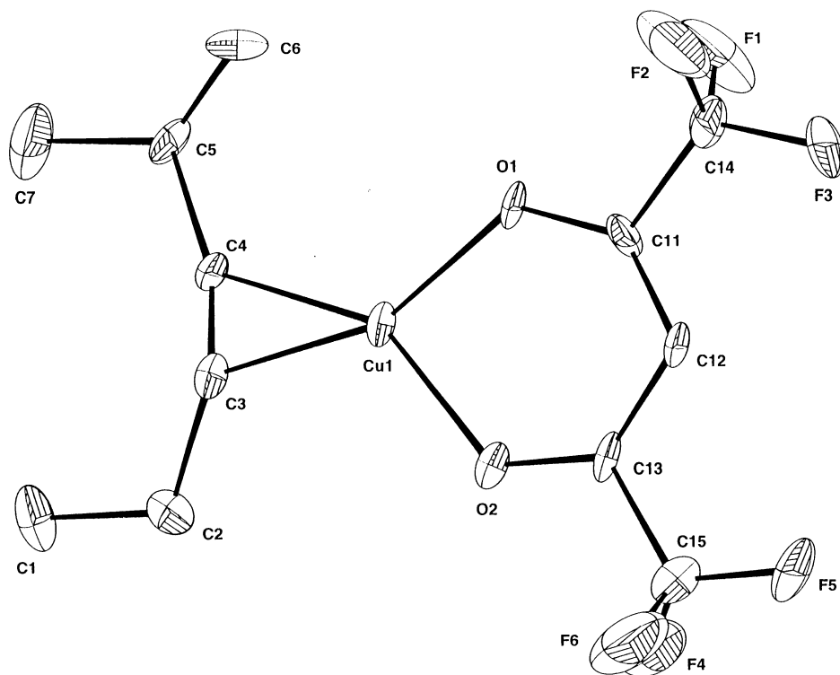
Fig. 5. ORTEP plot of (MHY)Cu(hfac) obtained by X-ray crystallographic analysis of a single crystal (J. Vaissermann et al., unpublished results).
