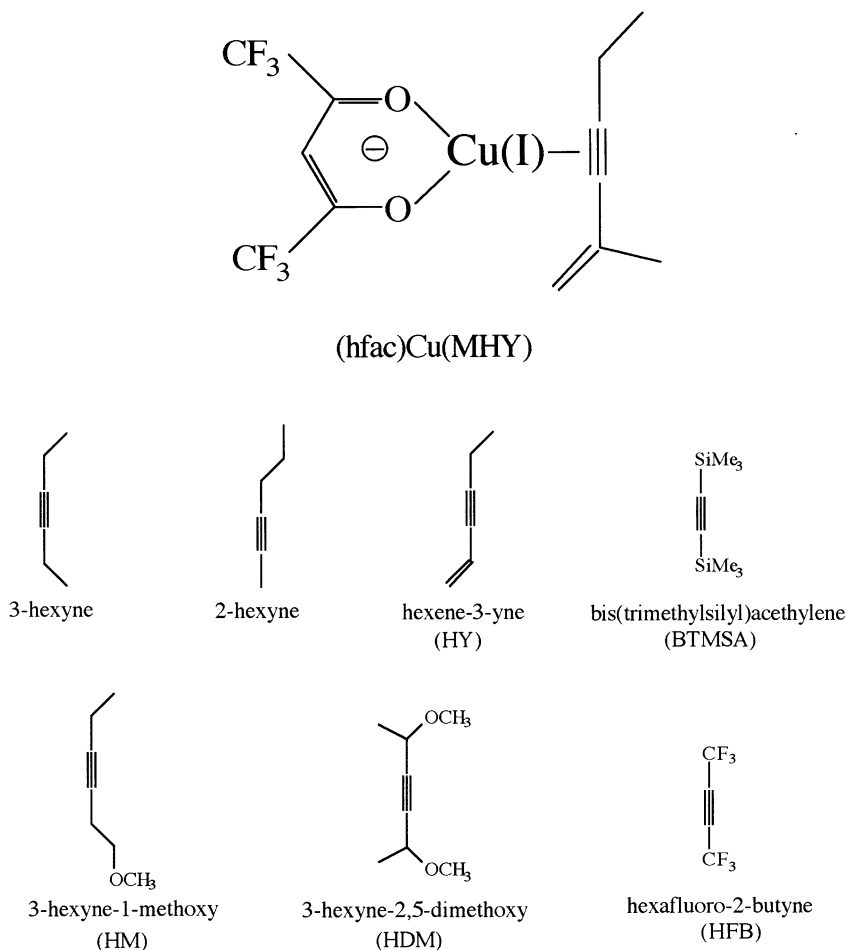
Fig. 4. Copper(I)( \text{hfac} ) Chemistries developed in this study. \text{MHY} can be substituted by VTMS (vinyltrimethylsilane), COD(cyclooctadiene), DMCOD (dimethyl-1,5-cyclooctadiene) or any alkyne present in the list except HFB (see text).
