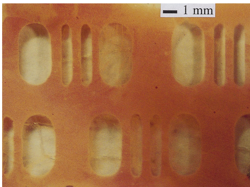
Fig. 9. Selective Cu CVD (using (MHY)Cu(hfac)) on \text{Si}_3\text{N}_4 film treated with IPTMS and UV irradiated through a mask. The copper film is \sim 400 nm thick.
